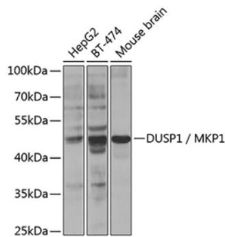
Fig. 1. Western blot analysis of extracts of various cell lines, using DUSP1 / MKP1 Antibody at 1:300 dilution. Secondary antibody: HRP-labeled Goat Anti-Rabbit IgG(H+L) (A0208) at 1:1000 dilution. Lysates/proteins: 25µg per lane. Blocking buffer: QuickBlock™ Blocking Buffer (P0231). Detection: BeyoECL Star (P0018A).
